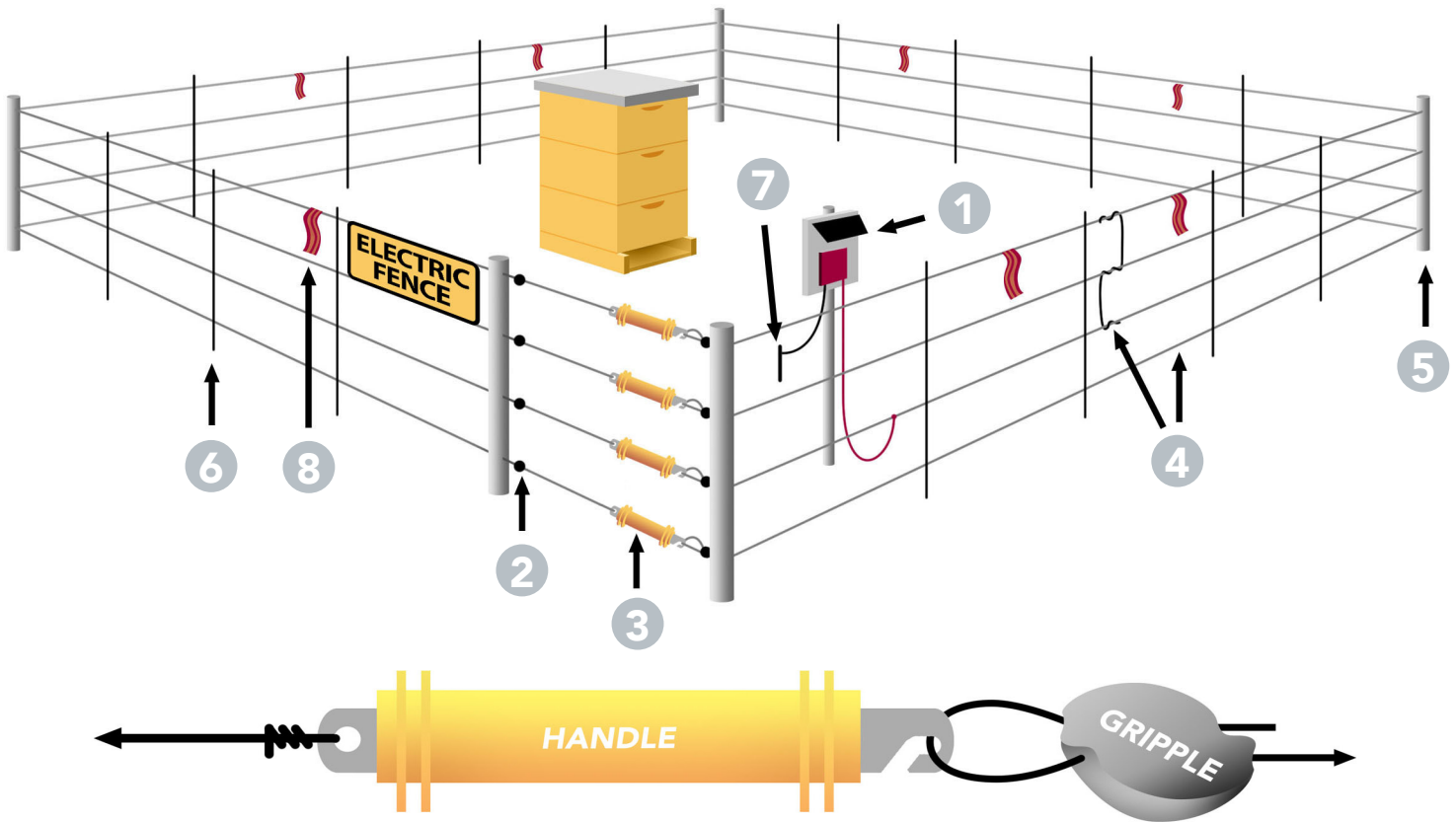
Gate Handle Detail: Gripple right against the corner post, loop of wire goes back through the gripple, loop hooks into existing gate handle hook, the other end of the handle gets attached with wire.
